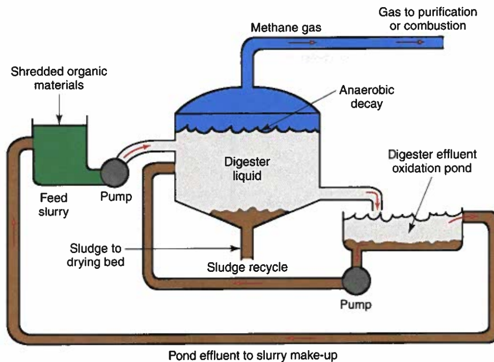
Figure 5-7. A methane digester produces usable methane gas from decaying organic matter.
